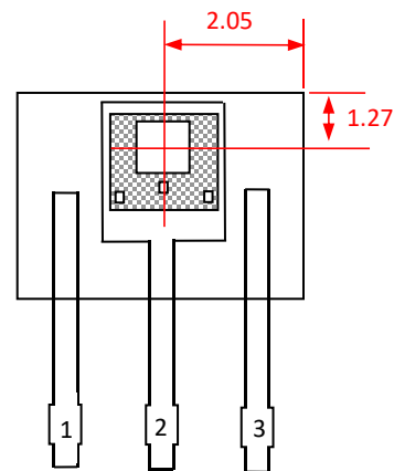
Sensor Location
