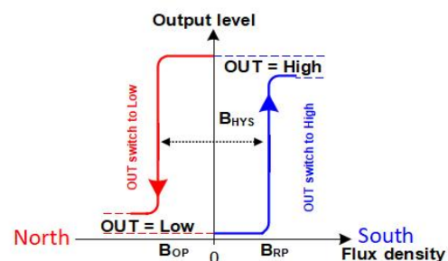
SO package - Latch characteristic
