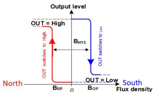
UA package - Latch characteristic
