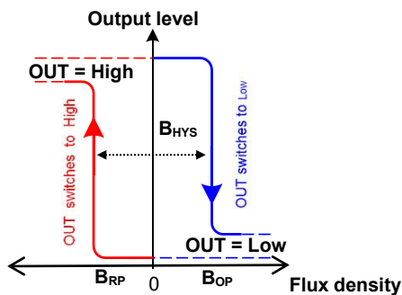
UA、DF package - Latch characteristic
