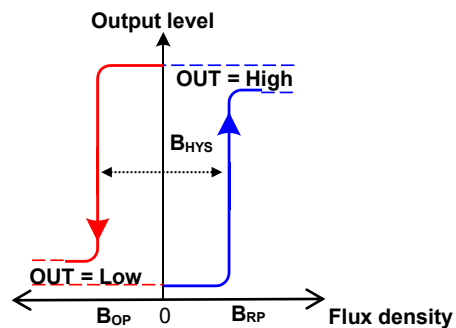
SO package - Latch characteristic
