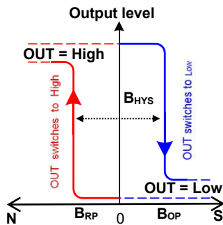
UA、DFN package - Latch characteristic
