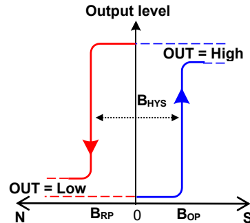
S0 package - Latch characteristic
